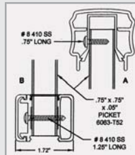
Intermediate Bracket
