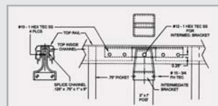
Intermediate Bracket
