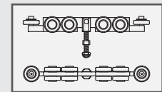
Detail - Trolley Assembly
