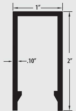
Privacy Horizontal Rail
