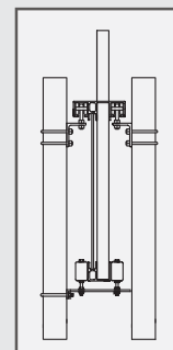
Track & Trolley Assembly (Double)
