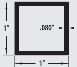
Security Picket
