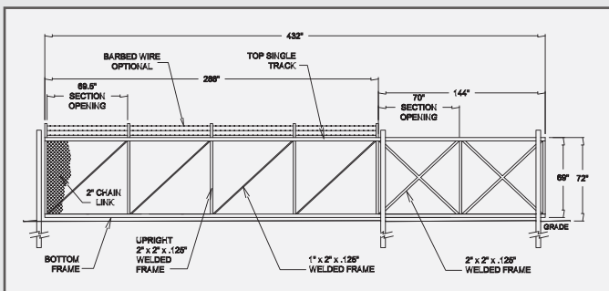
Chain Link Cantilever Gate (Detailed Example)
