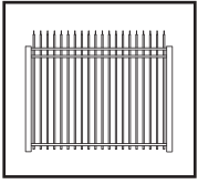
3 Channel
