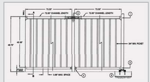
Guardrail Details
