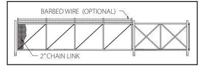
288" CANTILEVER • 6' CHAIN LINK
